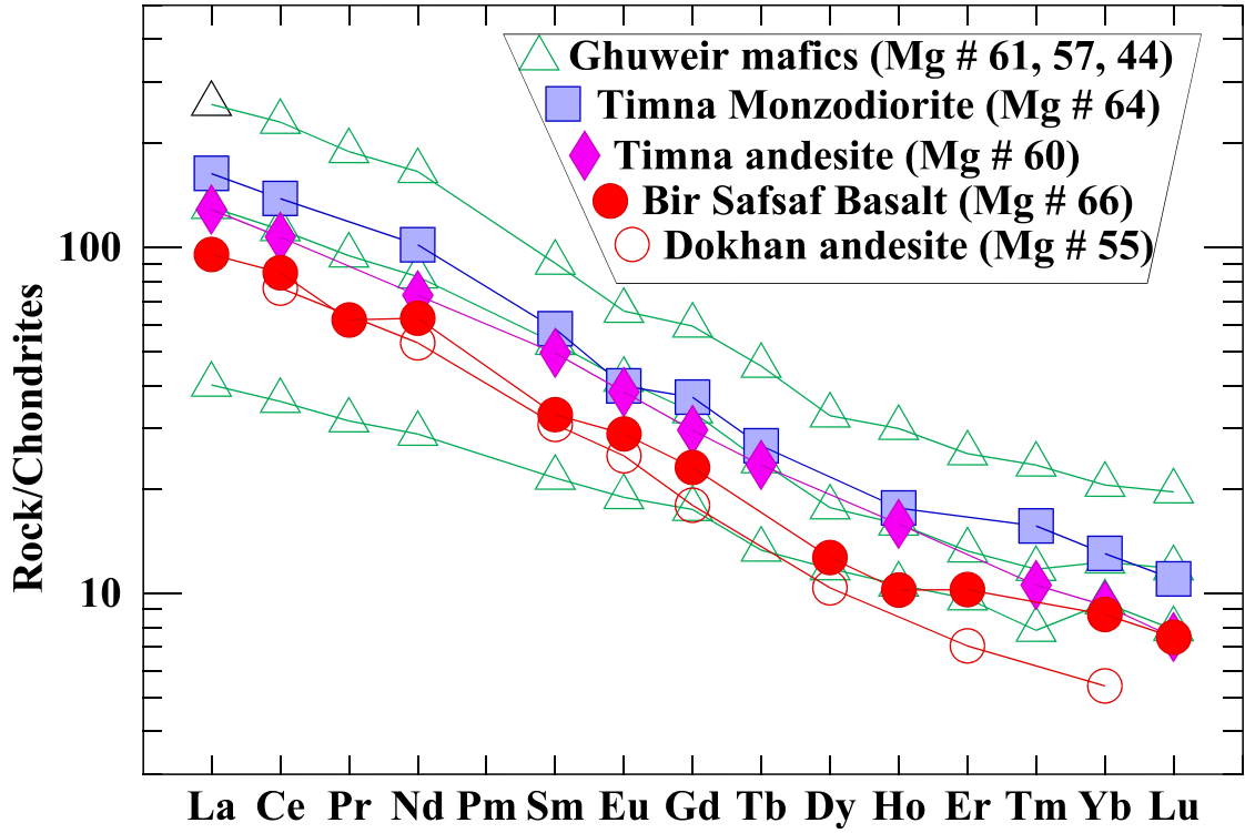
Figure 3. Chondrite-normalized Patterns for the Ghuweir Mafics and the Equivalent Rocks from the Adjacent Countries. The Mg #s are Calculated According to the Formula Mg \# = [\text{mol. prop. Mg}/(\text{mol. prop. Mg} + \text{mol. prop. Fe})] \times 100 .
